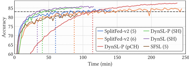
Figure 9: Evolution of accuracy through time when training ResNet18 on CIFAR10. Dashed vertical lines indicate the time-to-accuracy for accuracy 83%. For SplitFed-v2 and SFSL, we indicate in parentheses the number of client layers.
