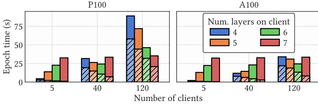
Figure 2: Epoch time (solid bars) and time during which the server GPU is actively training (bars with oblique hatches) when training ResNet18 with SplitFed-v1.
