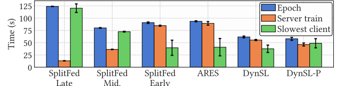
Figure 8: Breakdown of the epoch times when training EfficientNet with separate heads per client.
