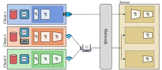
Figure 1: The optimal split depends on both compute and network. Client 2 trains more layers as it has a GPU; Client 3 (no GPU, slow WiFi) does too, but to exchange smaller embeddings; Client 1 (no GPU, fast link) trains fewer layers.
