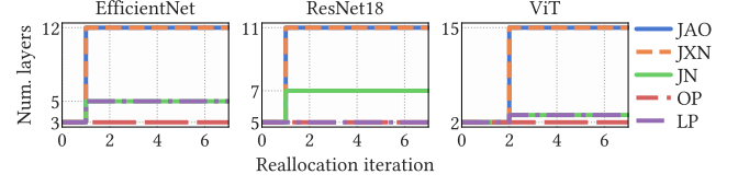
Figure 7: Allocated layers over an epoch with DynSL.
