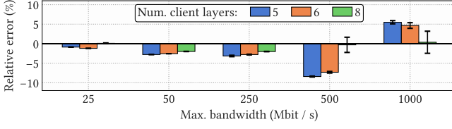
Figure 5: Relative error of bandwidth estimated by DynSL relative to iperf3 under various network regimes.
