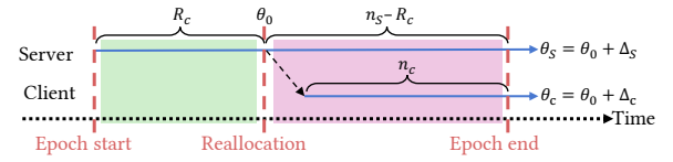
Figure 6: Example of migrating a layer within an epoch.
