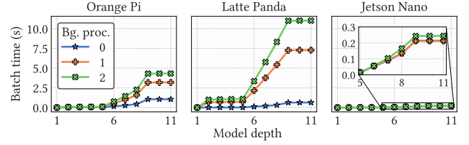
Figure 3: Training time under varying background loads.
