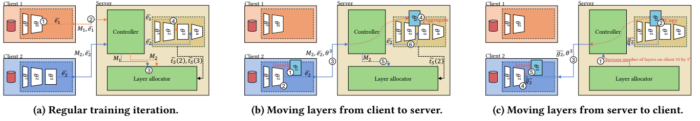
Figure 4: DYNsL overview. (4a): Clients ① run the forward pass and ② send embeddings ( \bar{e}_1, \bar{e}_2 ) and metrics ( M_1, M_2 ) to the server; the controller forwards ③ the metrics to the layer allocator and ④ embeddings to the model. (4b): When instructed to reduce its layers, the client ① detaches them, ② runs the forward pass through the reduced model, and ③ sends the removed weights with the next batch; the server ④ aggregates the client and server weights, ⑤ integrates the metrics, and ⑥ trains the model. (4c): To increase a client's layers, the allocator ① instructs the controller to ② extract the layer's current weights from the server and ③ send them with the gradients ( \bar{g}_2 ); the client ④ completes the backward pass, then ⑤ attaches the received layer.
