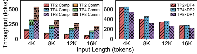
Figure 12. TP/DP tradeoff for Qwen3-8B-FP8 under TPOT_{p99} \leq 50 ms. The left panel stacks per-replica throughput by compute and communication share; the right panel shows eight-node aggregate throughput.
