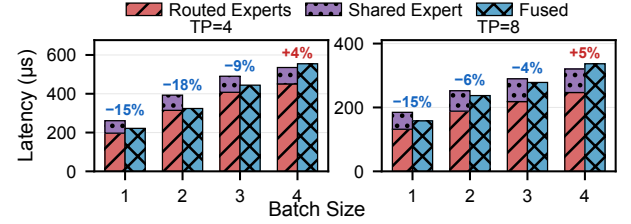
Figure 14. MoE expert fusion under TP-4 and TP-8. Fusion reduces small-batch overhead but regresses once larger batches amortize the unfused routed/shared expert kernels.
