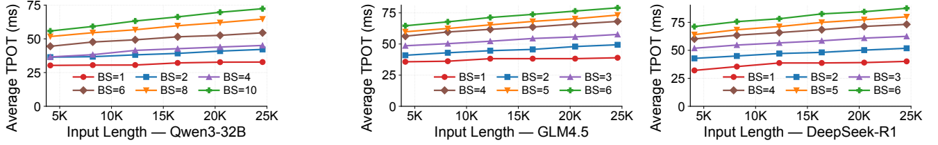
Figure 10. AMX TPOT microbenchmark across input length and batch size. Long-context TPOT remains bounded, but MoE models reach the TPOT limit at smaller batches than dense Qwen3-32B.
