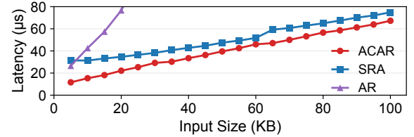
Figure 15. AllReduce latency. ACAR outperforms UCC’s SRA and AR for AMX decode’s small hidden-state messages. reduces latency from the best UCC latency of 26.5–74.9 \mu s to 11.6–67.3 \mu s, achieving a 1.1–2.3 \times speedup. These gains cover the small hidden-state messages issued by TP on the AMX decode path, showing that ACAR reduces latency for the decode collectives on CHORUS’s CPU lane.
