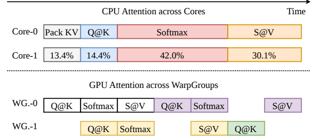
Figure 4. Attention core loop during decode. (a) CPU executes Pack-KV (AVX-512), QK^T (AMX), Softmax (AVX-512), and score \times V (AMX) in strict serial order; AMX tiles sit idle during the AVX-512 phases. (b) GPU asynchronously pipelines KV streaming with matmul and softmax, keeping Tensor Cores continuously occupied.
