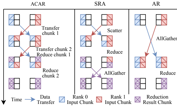
Figure 7. AllReduce designs. AVX-accelerated Chunk-pipelined AllReduce (ACAR) overlaps chunk transfer with AVX reduction; Reduce-Scatter AllGather (SRA) reduces distributed chunks before gathering them; AllGather Reduce (AR) gathers all chunks before local reduction.
