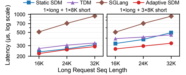
Figure 13. Decode MLA performance under mixed-length batches. Adaptive SDM balances cached-prefix work across cores, avoiding static-SDM stragglers and TDM serialization.
